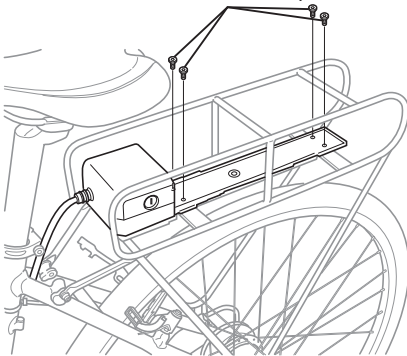
Hexagon socket head cap screw (M5) (not included with the product)
