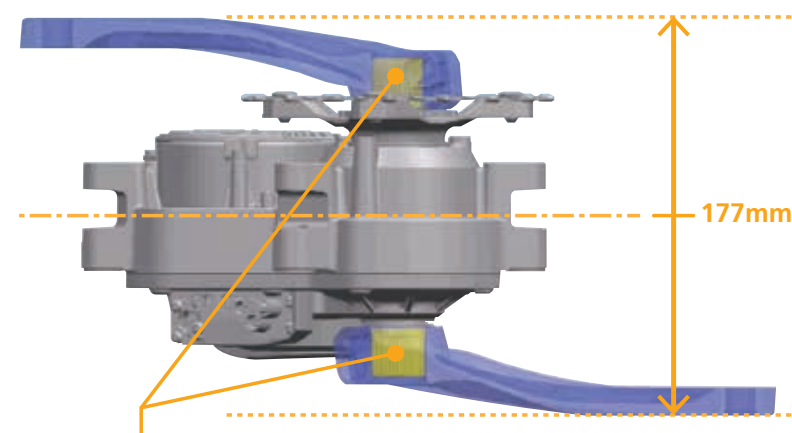
24mm Axle Serration
